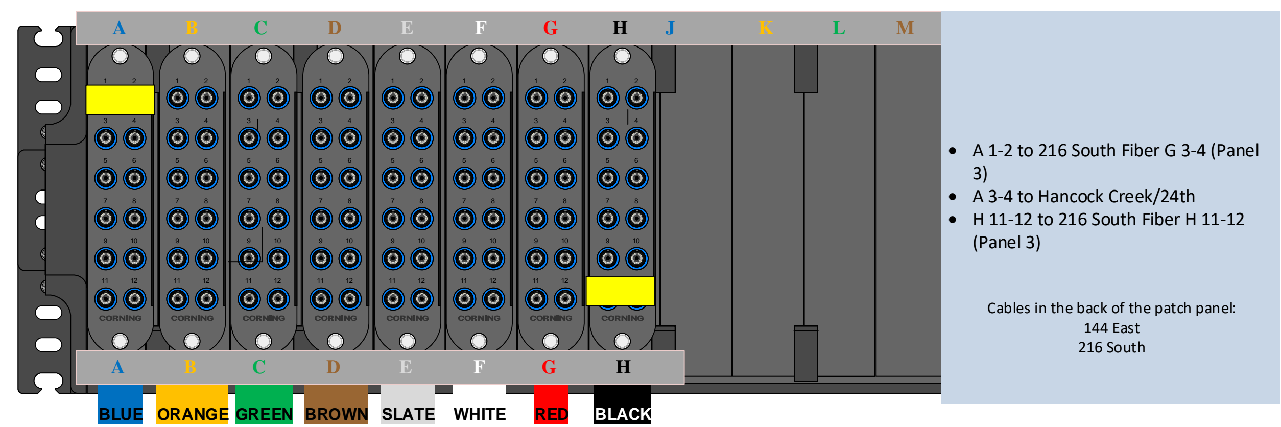
Del Prado @ Pine Island 144 East Fiber to Bus 41 Panel 2
