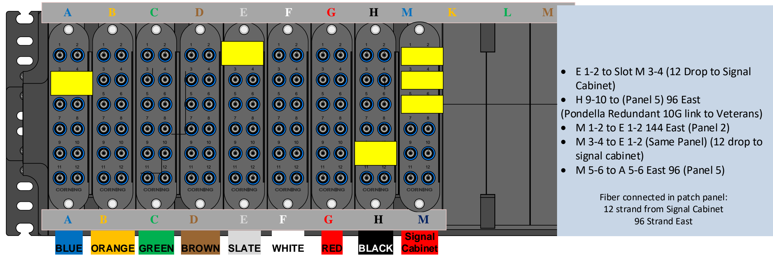
Del Prado @ Pine Island 96 North Panel 4
