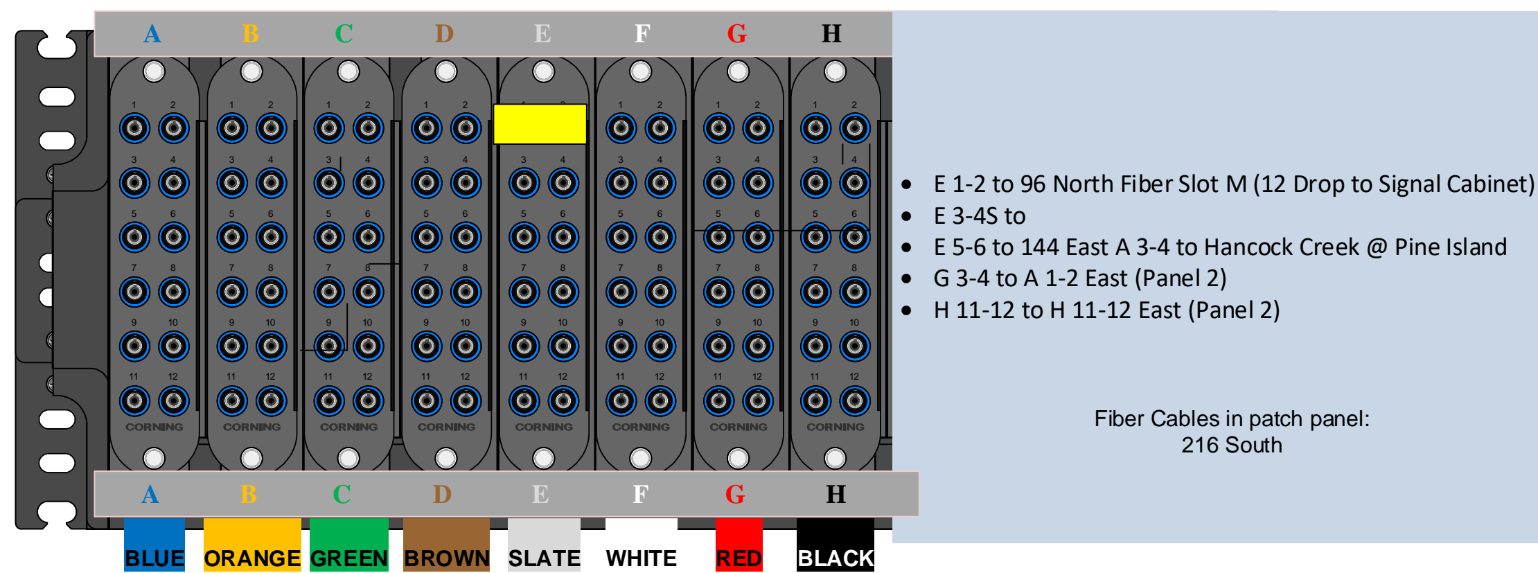
Del Prado @ Pine Island 216 South Fiber Panel 3
