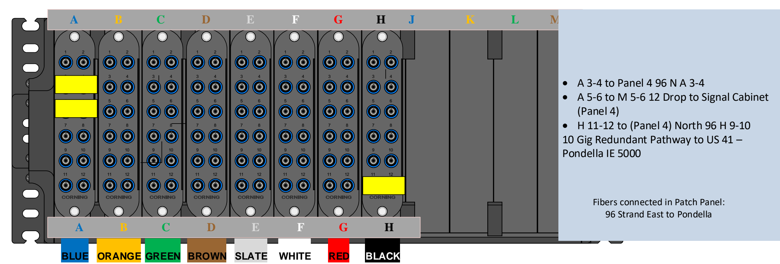
Del Prado @ Pine Island 96 East Fiber to Pondella Panel 5
