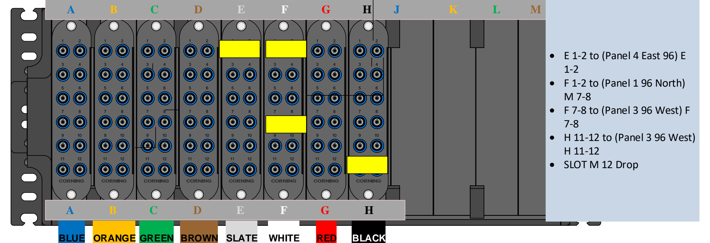
Bus 41 @ Pine Island 96 South Fiber Panel 5
