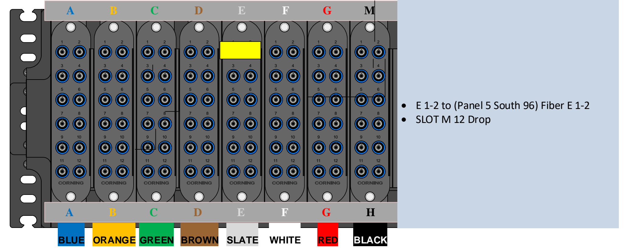
Bus 41 @ Pine Island 96 East Fiber Panel 4
