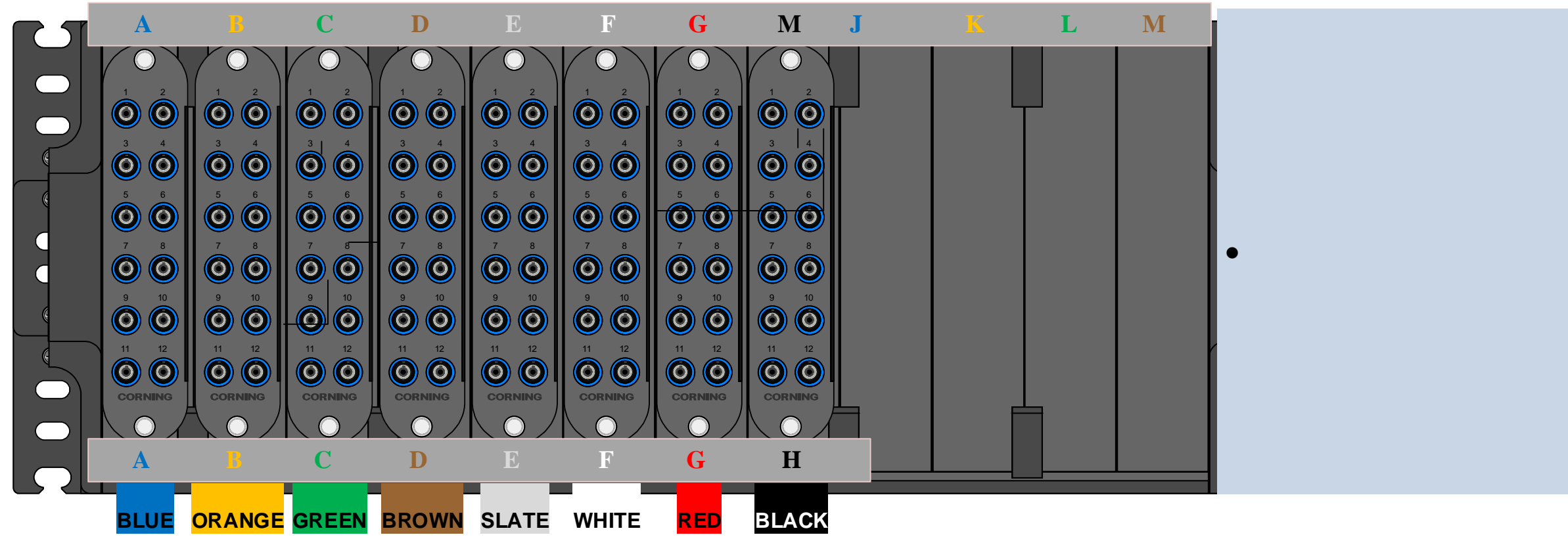
Bus 41 @ Pine Island 96 West Fiber 12F IMS SVS Panel 2
