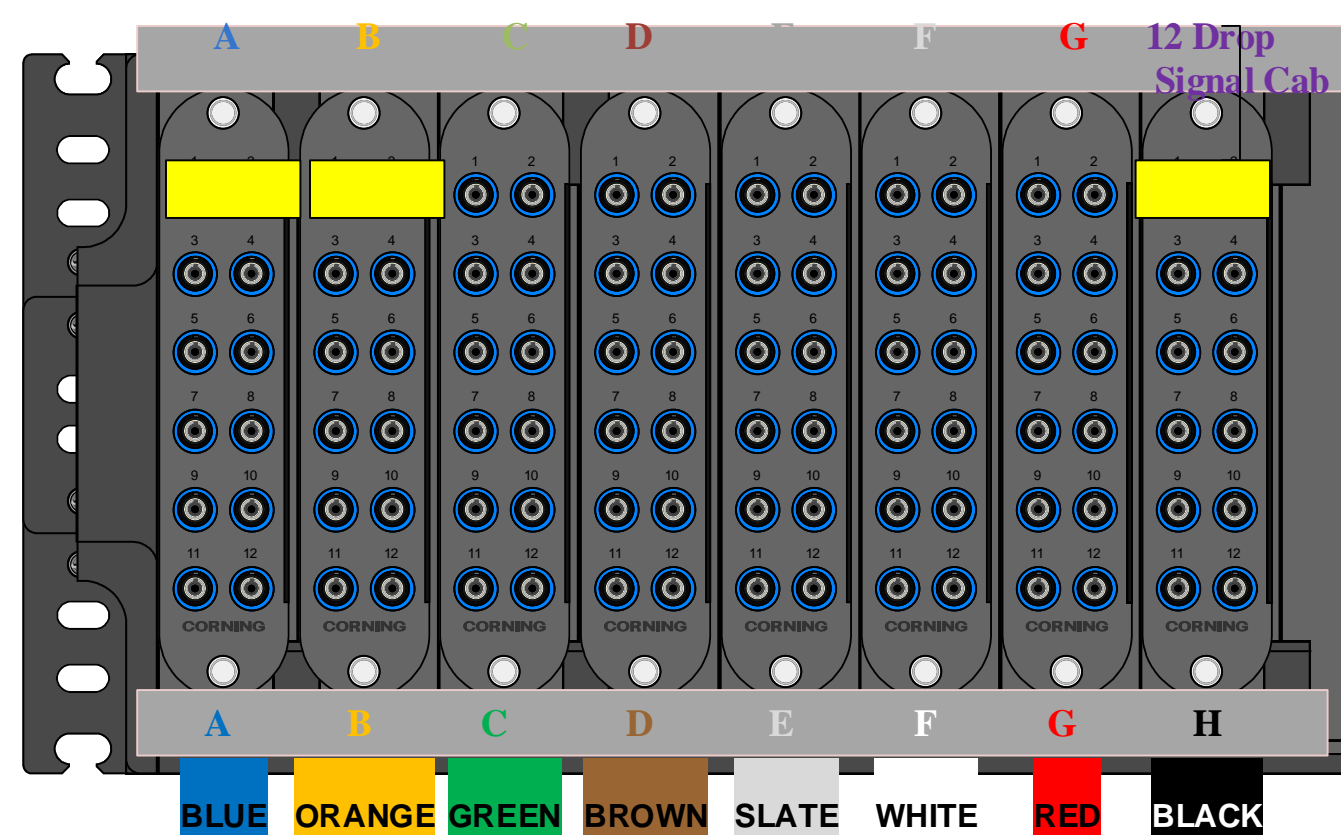
Del Prado @ Veterans Parkway 216 West Fiber
